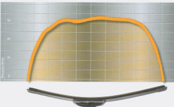
Pressure graph – Bosch Evolution™
