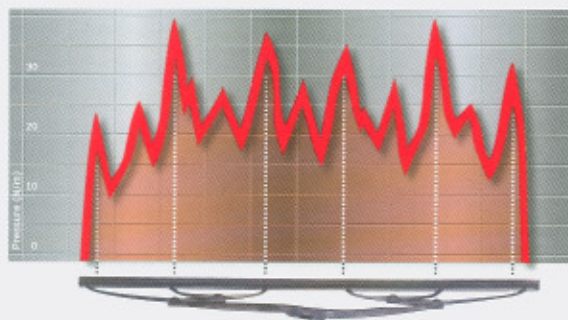
Pressure graph – conventional wiper blade
